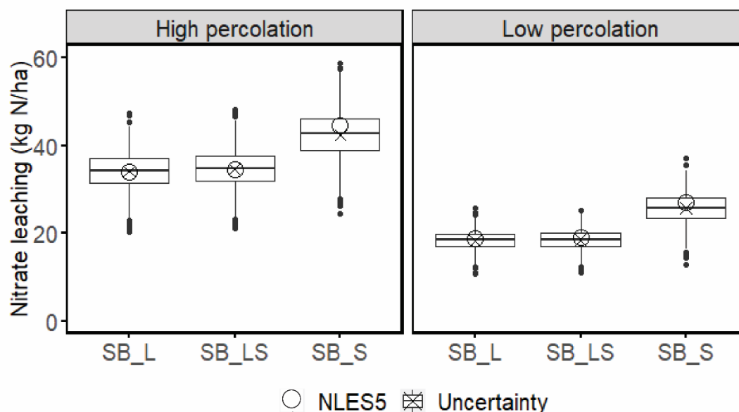
Figure 6.2. Effects of cover crops ( SB_B minus SB_{CC} ) obtained for the three soil types under two different percolation regimes. Boxes indicate the 25 to 75 percentile. Horizontal line within the box is the median. The uncertainty range is based on 1000 realisations of the NLES5 model reflecting the parameter uncertainties using a Monte Carlo approach. The upper and lower vertical lines from the hinge indicate the largest and smallest values at 1.5 \times IQR (where IQR is the inter-quartile range, or distance between the first and third quartiles, a roughly 95% confidence interval for comparing medians). Dots are observations outside the mean plus/minus the 95% confidence interval. \times is the mean value.
