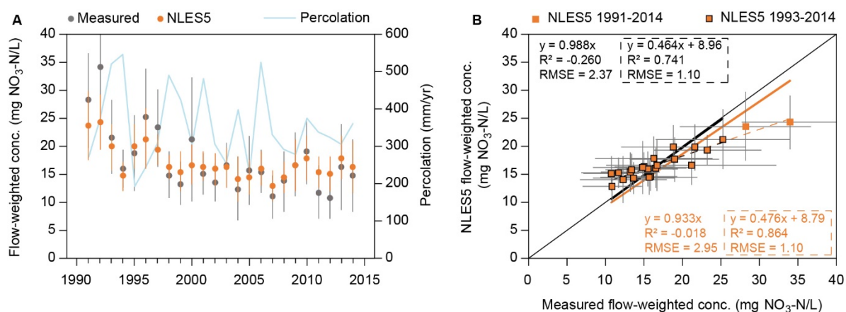
Figure 4.6. Measured and NLES5 predicted flow-weighted nitrate concentration as annual mean and standard deviation for LOOP data in the period 1991-2014; A) for the measured period, B x-y plot.
