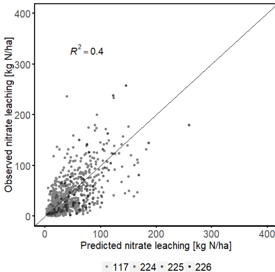
Figure 5.2. Observed versus model predicted annual nitrate leaching for the validation (Val) dataset shown separate for the four experiments. The line shows the 1:1 relation.
