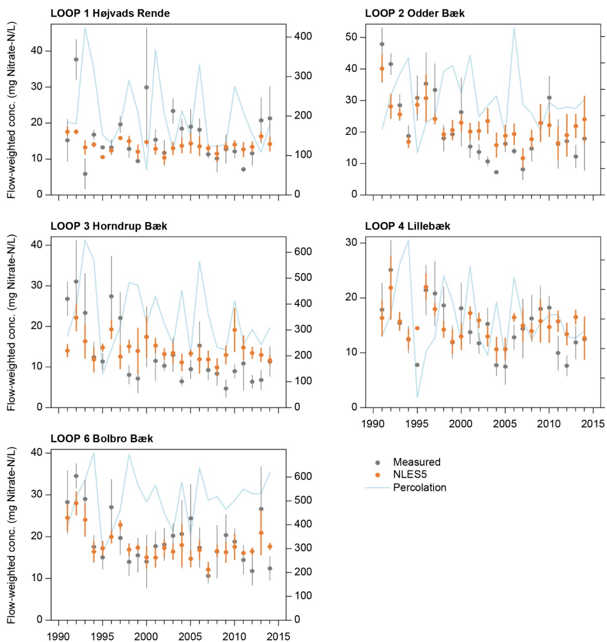
Figure 4.8. Measured and NLES5 predicted flow-weighted nitrate concentration and standard deviation for each of the five LOOP for the period 1991-2014. Note that the y-axes have different scale. The statistics of the relationship between observed and simulated mean annual N leaching is shown separately for each LOOP catchment.
