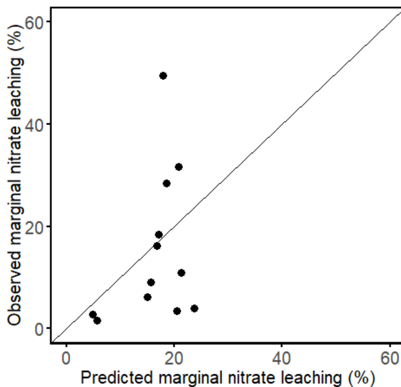
Figure 5.8. Observed versus model predicted marginal N leaching at standard fertilisation rate using data from experiment 226 for two different locations in the validation dataset (Val). Spring barley with cover crop and early sown winter wheat (Flakkebjerg) and winter rye (Foulum).
