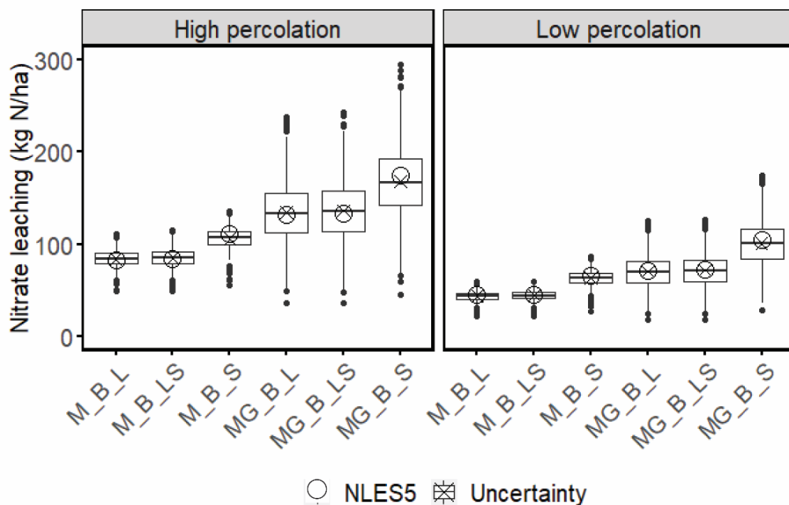
Figure 6.4. Field scale simulated nitrate leaching for two continuous crop rotation systems (M_B, maize followed by bare soil; and MG_B, maize after grass or grass-clover ploughed in spring followed by bare soil). Three soil types L (loam), SL (Sandy loam) and S (sand). The uncertainty range is based on 1000 realisations of the NLES5 model reflecting the parameter uncertainties using a Monte Carlo approach. Boxes indicate the 25 to 75 percentile. Two weather condition (High percolation and low percolation). The horizontal line within the box is the median. The upper and lower vertical lines from the hinge indicate the largest and smallest values at 1.5 \times IQR (where IQR is the inter-quartile range, or distance between the first and third quartiles, a roughly 95% confidence interval for comparing medians). Dots are observations outside the mean plus/minus the 95% confidence interval. \times is the mean value.
