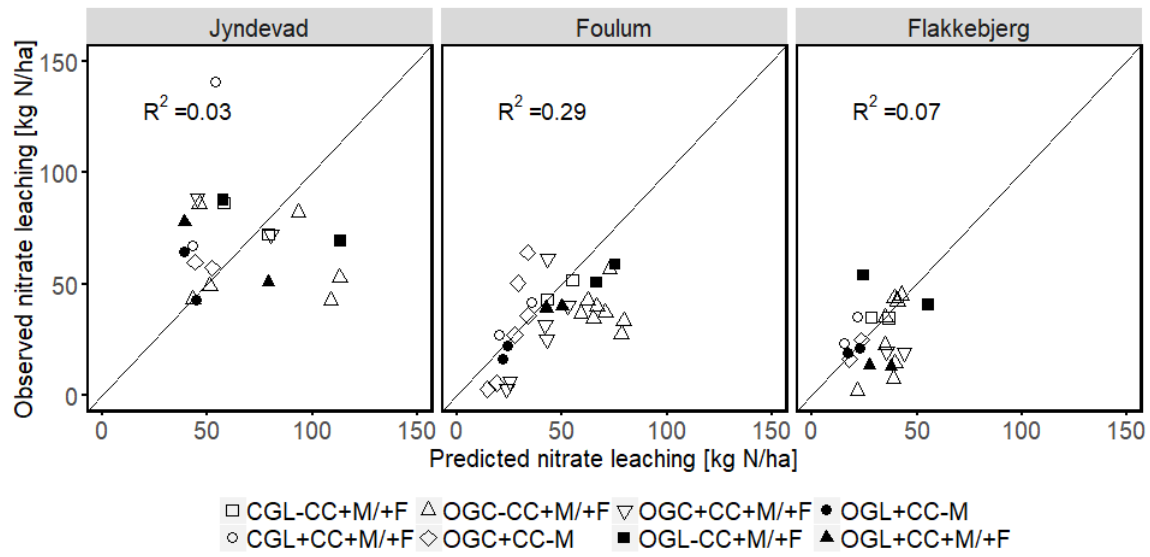
Figure 5.3. Observed versus predicted nitrate leaching as average over the period 2005-2008 from experiment 117 for three different locations. The long-term field experiments included (1) rotations with grass-clover in organic farming (OGC) or grain legumes in organic farming (OGL) or conventionally managed (CGL) systems, (2) with (+CC) and without (–CC) cover crops, and (3) with (+M) and without (–M) animal manure (in OGC and OGL), and with (+F) mineral fertilizer (in CGL). For details see Pandey et al. (2018).
