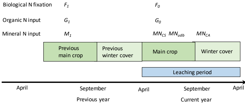
Figure 2.2. Timing of the crop and winter cover periods relative to the period defined for the nitrate leaching. The timing for N input in mineral and organic form from fertilization and biological N fixation is also shown for the current and previous year. In addition, NLES5 includes the N inputs from the year prior to the previous year (not shown in the graph).
