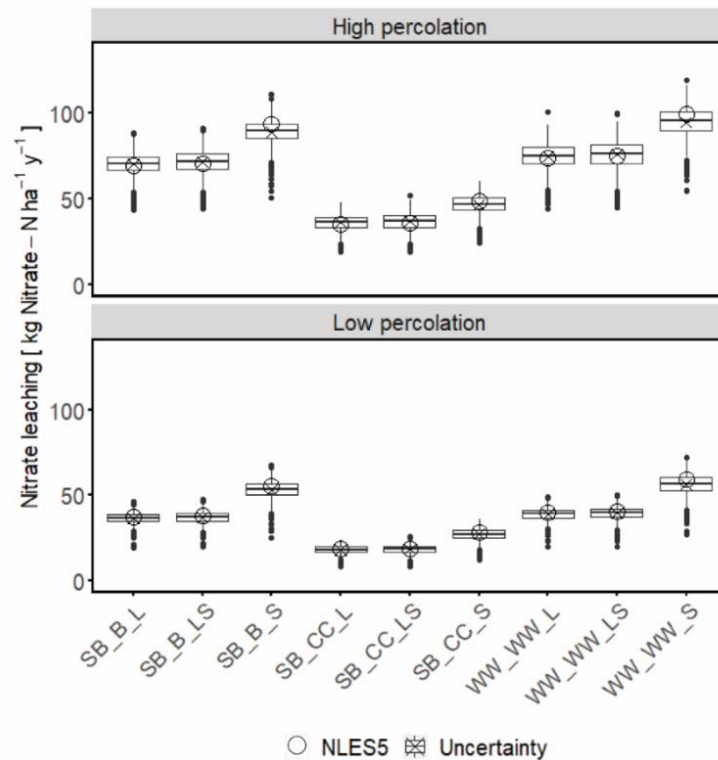
Figure 6.1. Field scale simulated nitrate leaching for three continuous crop rotations (SB_B, spring barley followed by bare soil; SB_CC, spring barley followed by catch crop; and WW_WW, winter wheat followed by winter wheat). Three soil types L (loam), SL (sandy loam) and S (sand). The uncertainty range is based on 1000 realisations of the NLES5 model reflecting the parameter uncertainties using a Monte Carlo approach. Boxes indicate the 25 to 75 percentile. Horizontal line within the box is the median. The upper and lower vertical lines from the hinge indicate the largest and smallest values at 1.5 \times IQR (where IQR is the inter-quartile range, or distance between the first and third quartiles, a roughly 95% confidence interval for comparing medians). Dots are observations outside the mean plus/minus the 95% confidence interval. \times is the mean value.
