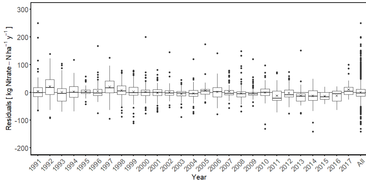
Figure 4.2. Residuals (observed minus model predicted) nitrate leaching over the years 1991-2017 (Cal1 dataset). The horizontal lines in the box indicate the median values, and the lower and upper hinges correspond to the first and third quartiles (the 25th and 75th percentiles). The upper and lower vertical lines from the hinge indicate the largest and smallest values at 1.5 * IQR , where IQR is the inter-quartile range, corresponding to the 95% confidence interval. \times shows the mean.
