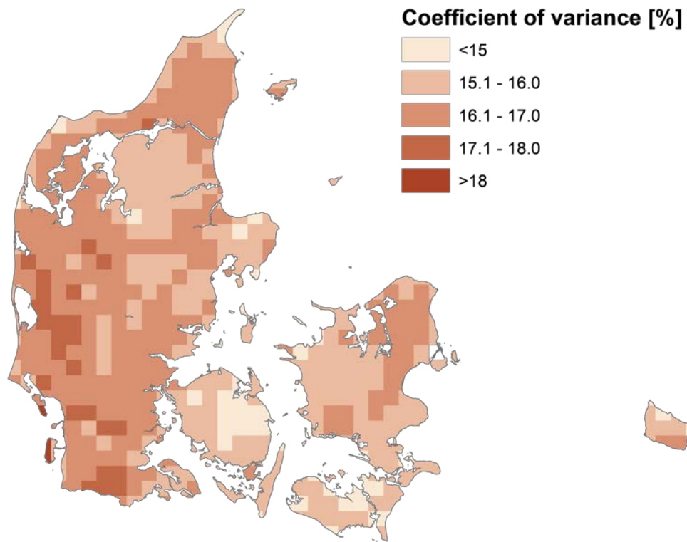
Figure 6.9. Coefficient of variance (%) of parameter uncertainty for the marginal N leaching based on model predictions using 1000 different sets of NLES5 parameter data sets. The uncertainty range is based on 1000 realisations of the NLES5 model reflecting the parameter uncertainties using a Monte Carlo approach.
