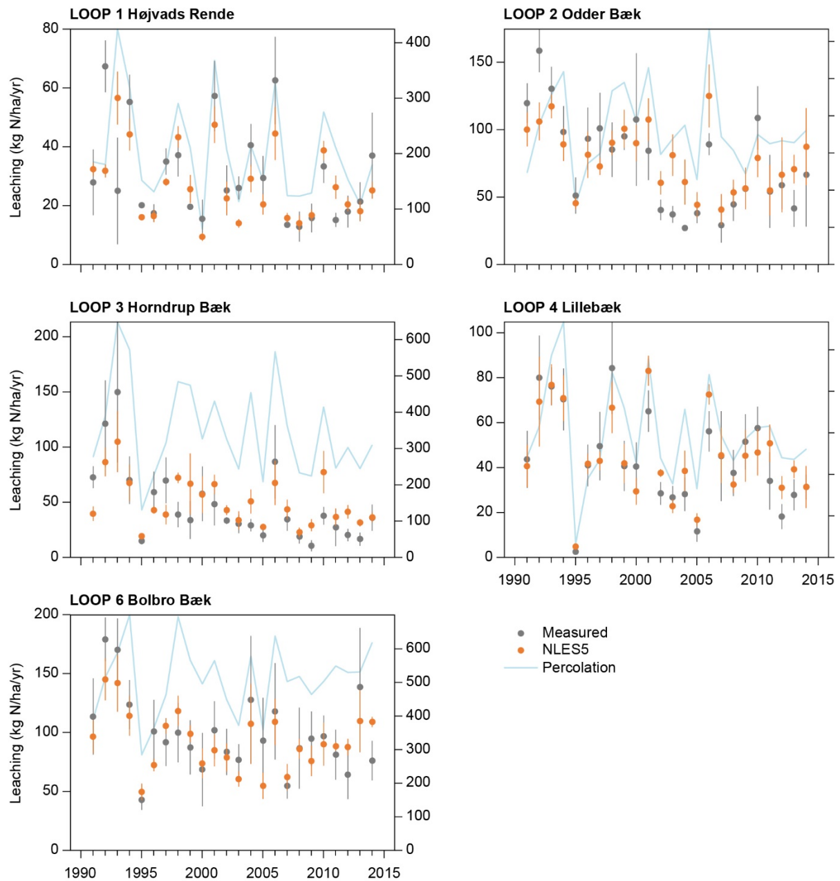
Figure 4.7. Measured and NLES5 predicted nitrate leaching (kg N/ha) as annual mean and standard deviation for each of the five LOOP catchments in the period 1991-2014. Note that the y-axes have different scales. The statistics of the relationship between observed and simulated mean annual N leaching is shown separately for each LOOP catchment.
