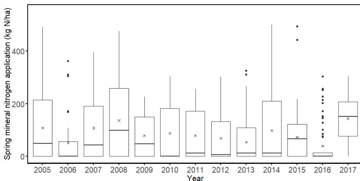
Figure 2.6. Mineral N application rates for the validation data set. Vertical lines indicate the standard deviation. Boxes indicate the 25 to 75 percentile. The horizontal line within the box is the median. The upper and lower vertical lines from the hinge indicate the largest and smallest values at 1.5 * IQR , where IQR is the inter-quartile range, or distance between the first and third quartiles, a roughly 95% confidence interval for comparing medians. Dots are observations outside the mean plus/minus the 95% confidence interval. \times is the mean value.
