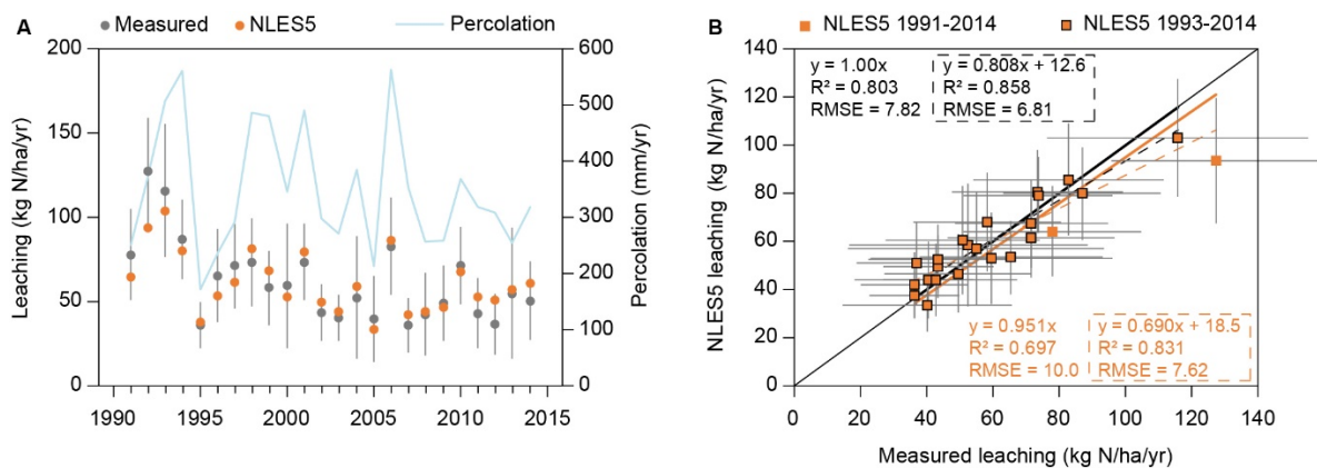
Figure 4.5. Measured and NLES5 predicted nitrate leaching as annual mean and standard deviation for the five LOOP catchments in the period 1991-2014, A) annual values, B) x-y plot. Annual percolation is shown in A.
