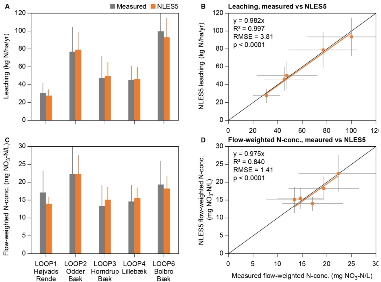
Figure 4.4. Average and standard deviation for measured and NLES5 predicted nitrate leaching (A) and (C) for each of the five LOOP catchments, x-y plot for leaching (B) and flow-weighted nitrate concentrations (D) for the average value calculated for the period 1991-2014.
