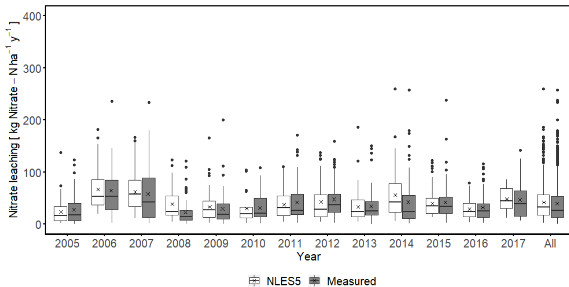
Figure 5.1. Observed and model predicted nitrate leaching over the period 2005-2017 for model validation (Val dataset). The horizontal lines in the box indicate the median values, and the lower and upper hinges correspond to the first and third quartiles (the 25th and 75th percentiles). The upper and lower vertical lines from the hinge indicate the largest and smallest values at 1.5 * IQR , where IQR is the inter-quartile range, corresponding to the 95% confidence interval. \times shows the mean.
