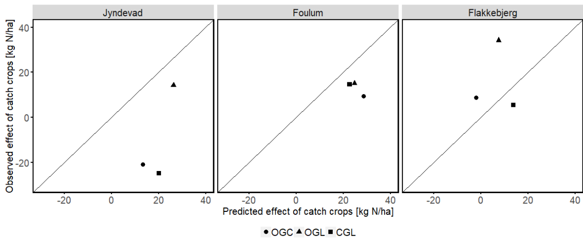
Figure 5.5. Observed versus predicted nitrate leaching effects of cover crops at cropping system level for 2005-2008 from experiment 117 for three different locations. The symbols refer to the different cropping systems as defined by Pandey et al. (2018). For details see caption of Figure 5.3. Cover crops in OGC and OGL included a mixture of perennial ryegrass and clover (at the sites with coarse sand and sandy loam soils) or winter rye, fodder radish and vetch (at the site with loamy sand soil), and cover crops in CGL included only perennial ryegrass at all the sites.
