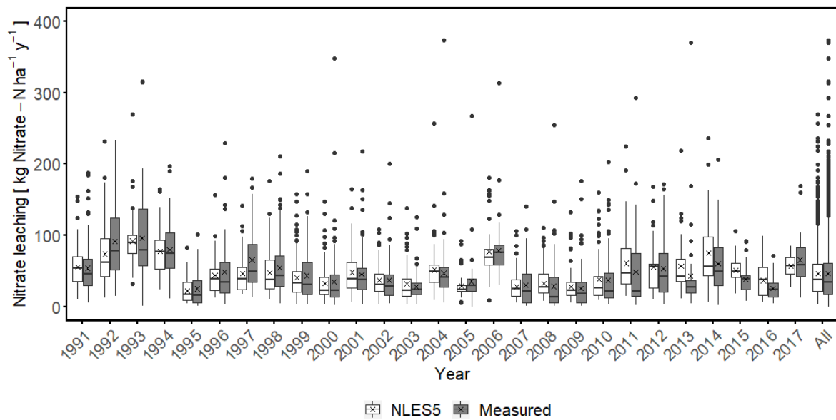
Figure 4.1. Observed and model predicted nitrate leaching over the period 1991-2017 ( Cal1 dataset). The horizontal lines in the box indicate the median values, and the lower and upper hinges correspond to the first and third quartiles (the 25th and 75th percentiles). The upper and lower vertical lines from the hinge indicate the largest and smallest values at 1.5 * IQR , where IQR is the inter-quartile range, corresponding to the 95% confidence interval. \times shows the mean.
