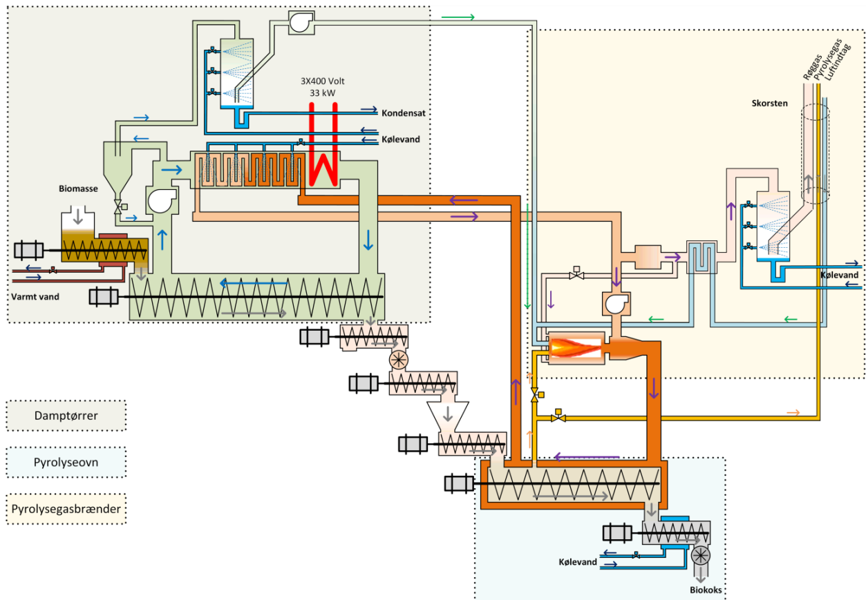
Figure 2.13. Diagram of a combined sludge and pyrolysis plant from AquaGreen. From Odsherred Kommune (2021). Damptrørrer = steam dryer; Pyrolyseovn = pyrolysis reactor; Pyrolysegasbrænder = pyrolytic gas burner; Kølevand = cooling water; Biokoks = biochar.
